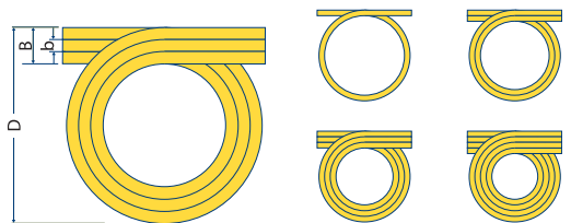
Top view dimensions Single, 2, 3 & 4 track
