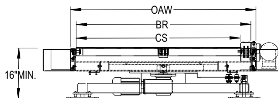
MAXIMUM LOAD 2500 LBS.
